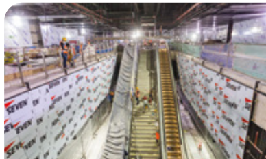
Ongoing testing and commissioning of escalators in preparation for Jabatan Keselamatan dan Kesihatan Pekerjaan (JKKP) inspection at the platform level of the Raja Uda MRT Station.
