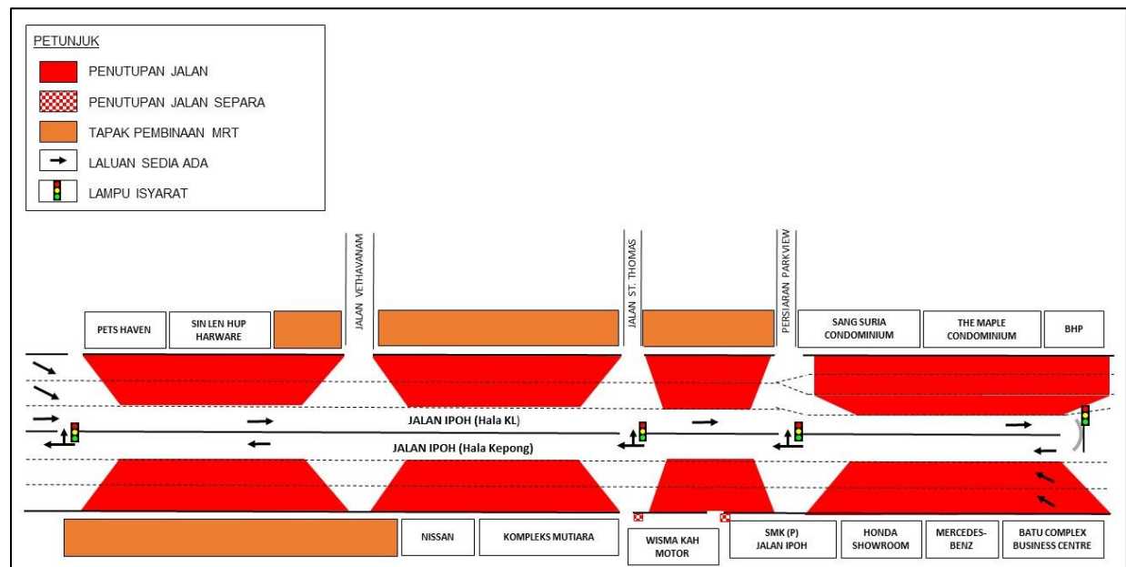
MAP 1(a) : CONTINUATION OF NIGHT LANE CLOSURES ALONG JALAN IPOH – NEAR KOMPLEKS MUTIARA (KL-BOUND AND KEPONG-BOUND)
