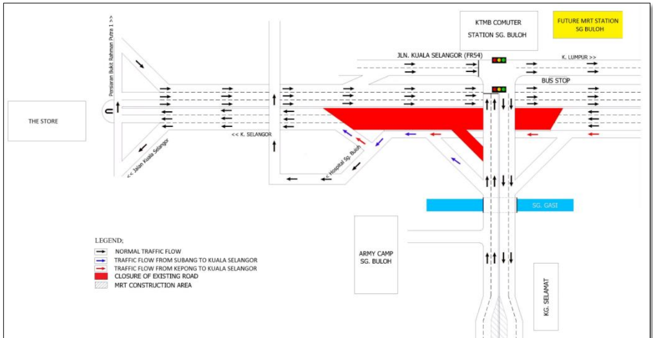
MAP (i) CLOSURE A: CLOSURE OF 300M STRECTH ROAD AT JALAN KUALA SELANGOR-KEPONG (KUALA SELANGOR-BOUND)
