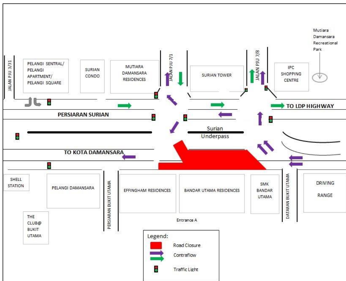
MAP 2: PHASE 2 TRAFFIC MANAGEMENT PLAN FOR PERSIARAN SURIAN AT MUTIARA DAMANSARA
