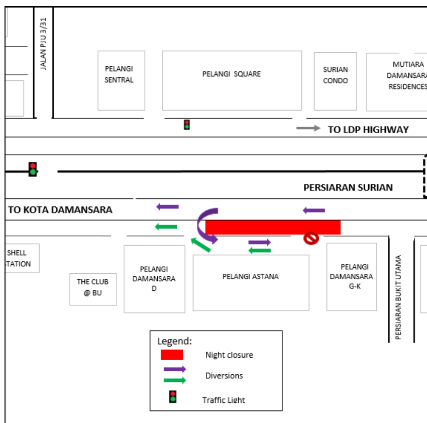
MAP 2 (PHASE 2): LAUNCHING OF TRUSS
