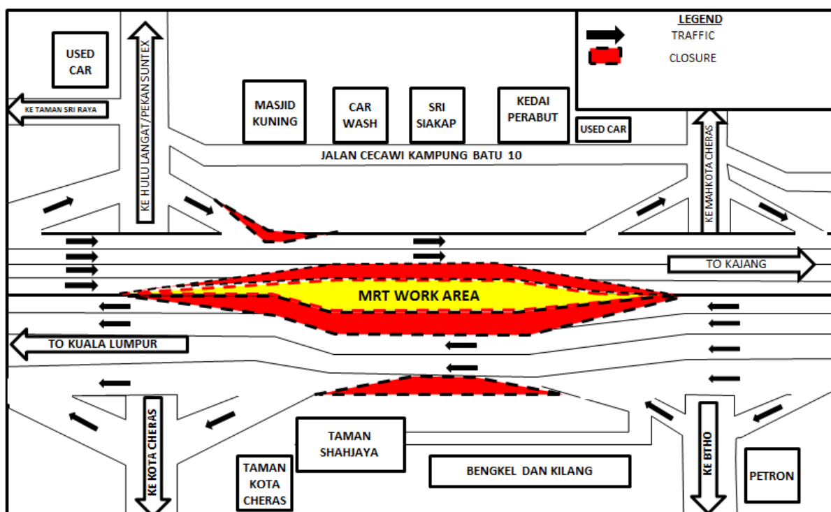
MAP 8: CONTINUATION OF LANE CLOSURE AT KM 14.4 UNTIL KM 14.8 ON CHERAS-KAJANG HIGHWAY (KAJANG-BOUND AND KUALA LUMPUR-BOUND)
