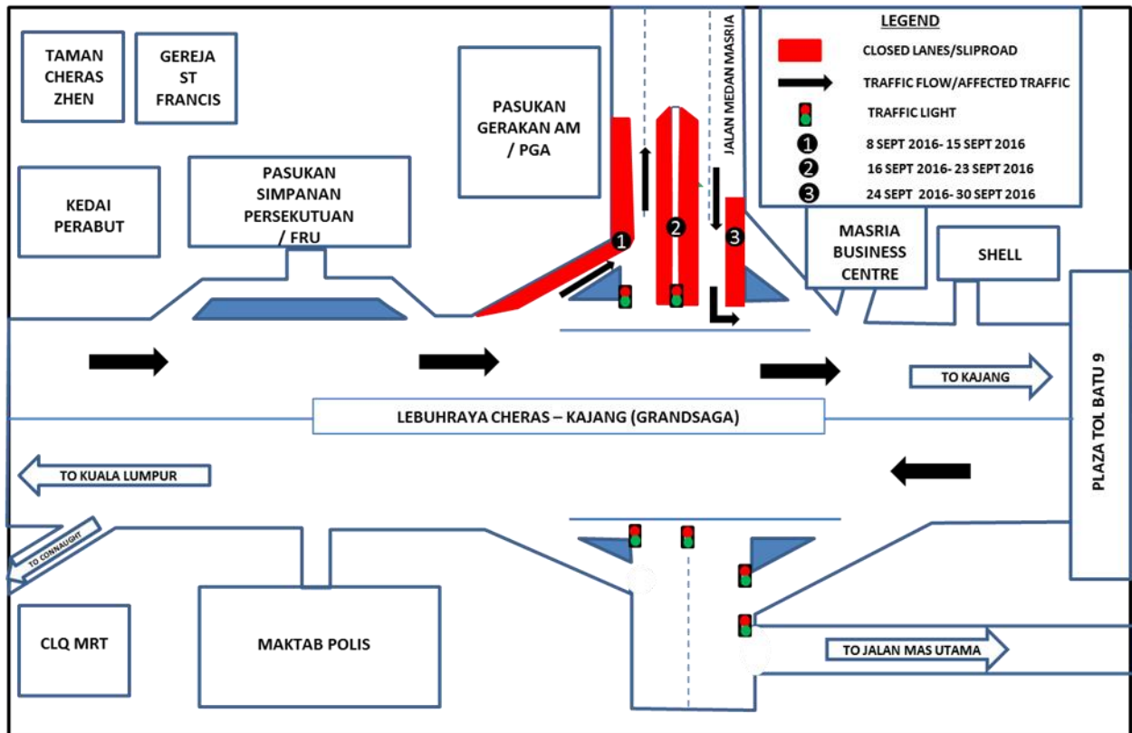
MAP 14 - CONTINUATION OF PARTIAL LANE CLOSURE AT EXIT 701 – PGA INTERCHANGE CHERAS KAJANG HIGHWAY
