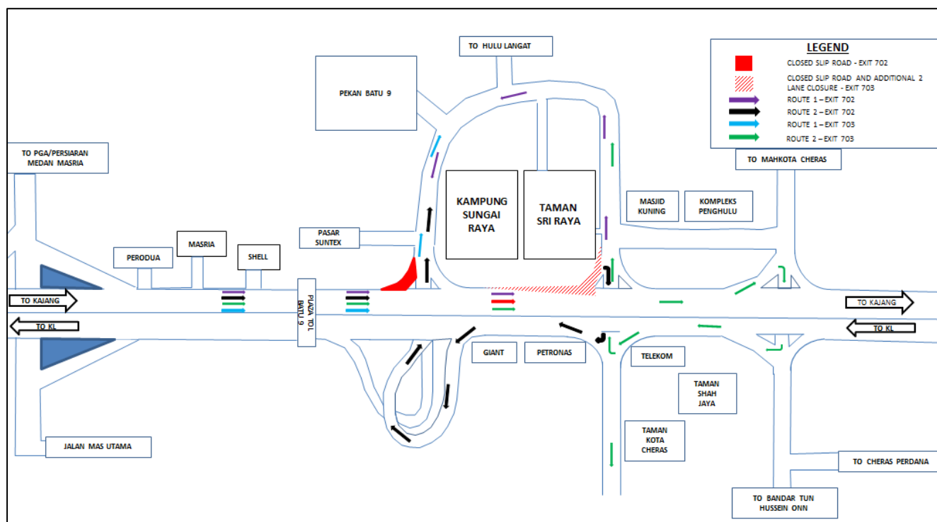
MAP 9: CONTINUATION OF SLIP ROAD CLOSURES AT EXIT 702 AND EXIT 703, CHERAS-KAJANG HIGHWAY (KAJANG –BOUND AND KUALA LUMPUR-BOUND)
