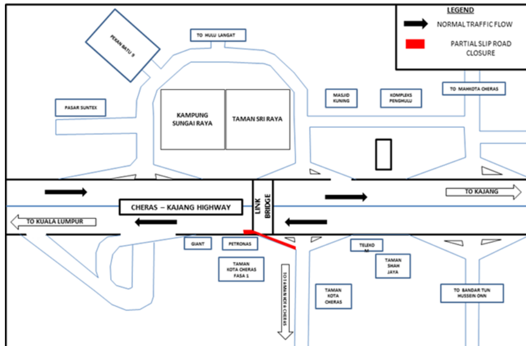
MAP 8: CONTINUATION OF PARTIAL LANE AND SLIP ROAD CLOSURE AT EXIT 703 – TELEKOM INTERCHANGE ON CHERAS-KAJANG HIGHWAY (KUALA LUMPUR BOUND)
