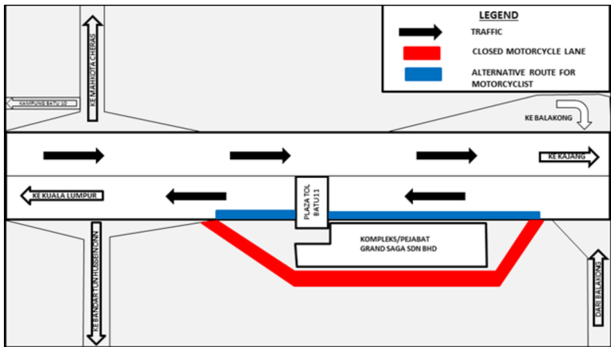
MAP 6: CONTINUATION ON MOTORCYCLE LANE CLOSURE AT BATU 11 TOLLBOOTH OF CHERAS – KAJANG HIGHWAY (KUALA LUMPUR AND KAJANG BOUND)
