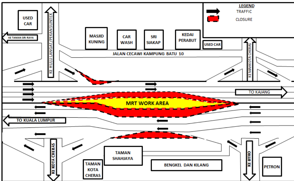
MAP 1: CONTINUATION OF FULL LANE CLOSURE AT KM 14.4 UNTIL KM 14.8 ON CHERAS-KAJANG HIGHWAY (KAJANG-BOUND AND KUALA LUMPUR-BOUND)
