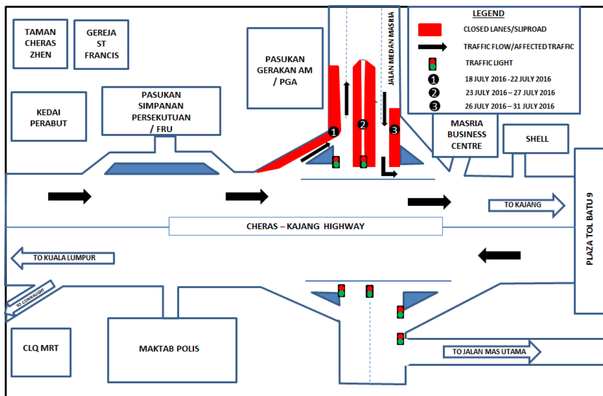
MAP 7: CONTINUATION ON PARTIAL LANE CLOSURE AT EXIT 701 – PGA INTERCHANGE CHERAS-KAJANG HIGHWAY (KAJANG BOUND)
