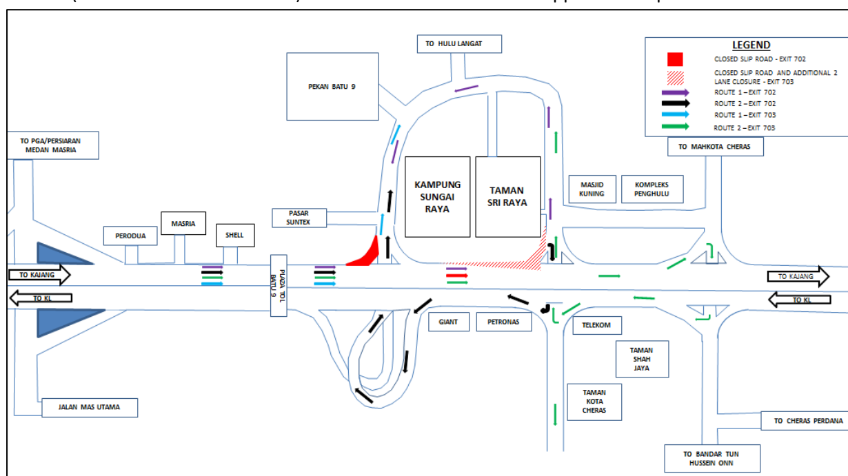
MAP 8 - CONTINUATION OF SLIP ROAD CLOSURE AT THE EXIT 702 AND EXIT 703, CHERAS KAJANG HIGHWAY
