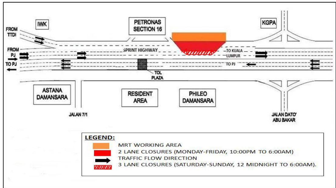
MAP 6: CONTINUATION OF LANE CLOSURE AT SPRINT HIGHWAY AFTER PETRONAS STATION, SECTION 16 (KL-BOUND)
