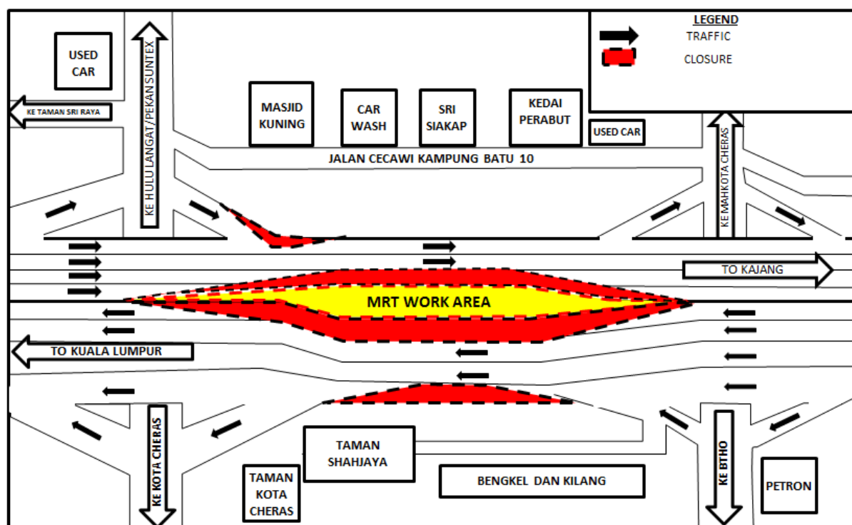
MAP 7: LANE CLOSURE AT KM 14.4 UNTIL KM 14.8 ON CHERAS KAJANG HIGHWAY (KAJANG AND KUALA LUMPUR BOUND).
