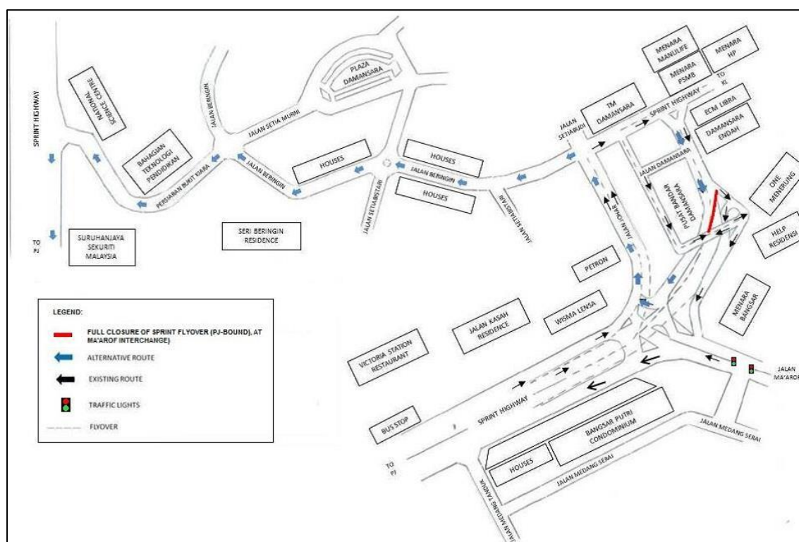
MAP 3: CONTINUATION OF FULL ROAD NIGHT CLOSURE OF SPRINT HIGHWAY NEAR PUSAT BANDAR DAMANSARA (PJ-BOUND)
