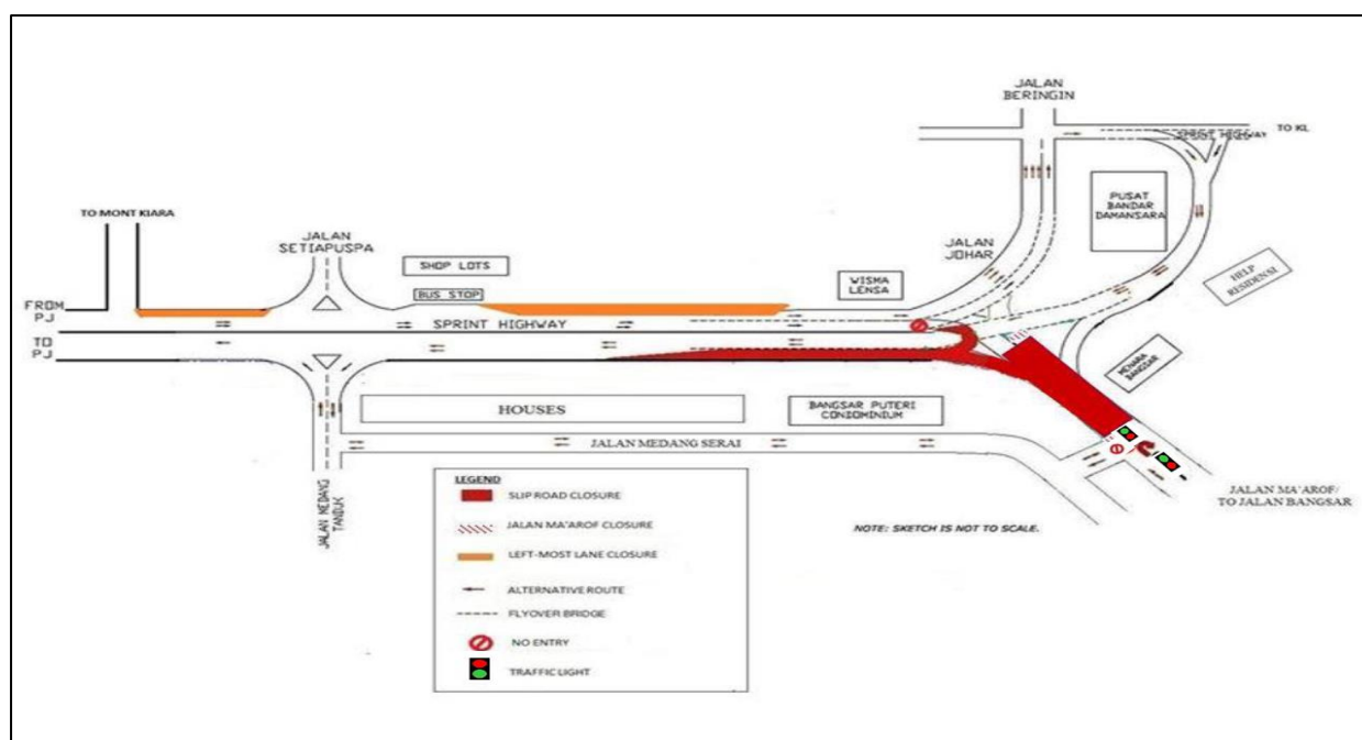
MAP 4: CONTINUATION OF NIGHT TRAFFIC MANAGEMENT AT SPRINT HIGHWAY AND JALAN MA'AROF (KL AND PJ-BOUND)
