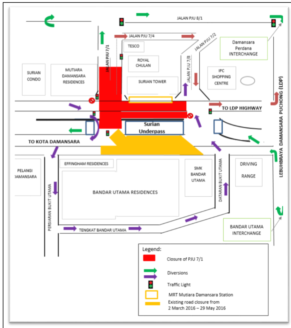
MAP 1 .TRAFFIC MANAGEMENT PLAN AT PJU 7/1 FOR INSTALLATION OF LINK BRIDGE IN THE VICINITY OF MUTIARA DAMANSARA. PERSIARAN SURIAN
