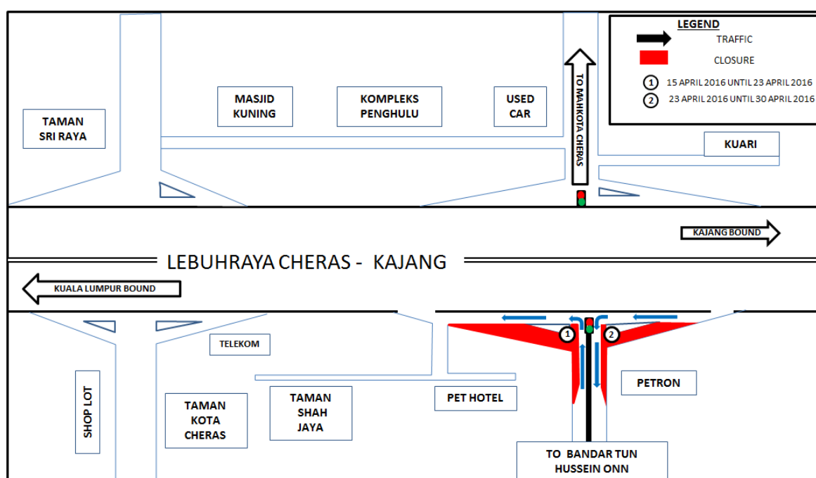
MAP 2: PARTIAL LANE AND SLIP ROAD CLOSURE AT EXIT 704 – BANDAR TUN HUSSEIN ONN INTERCHANG CHERAS-KAJANG HIGHWAY
