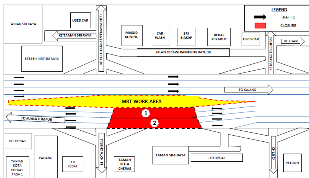
MAP 4: TEMPORARY LANE CLOSURE AT KM 14.0 UNTIL KM 14.7, LEBUHRAYA CHERAS - KAJANG (KUALA LUMPUR-BOUND)
