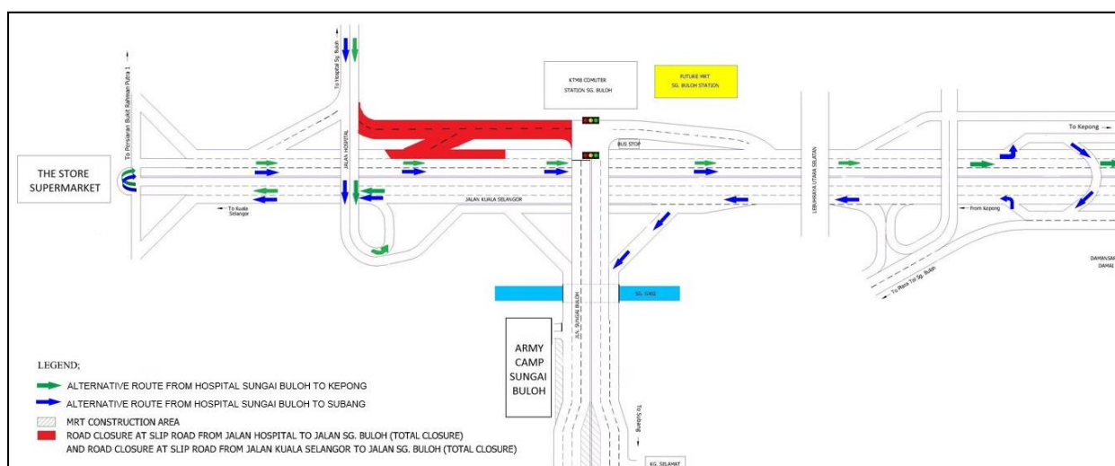
MAP 7 ( i ): ROAD CLOSURE AT SLIP ROAD FROM JALAN HOSPITAL UNTIL THE TRAFFIC LIGHT OF JALAN SUNGAI BULOH (SUBANG-BOUND)/JALAN KUALA SELANGOR (KEPONG-BOUND)
