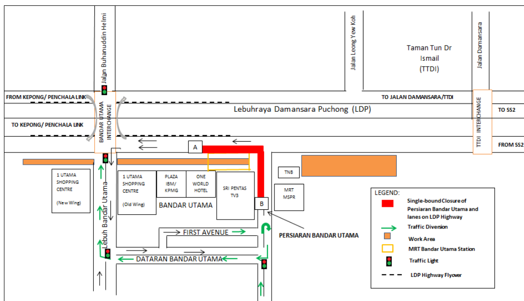
MAP 3: CONTINUATION OF LONG-TERM NIGHT TRAFFIC MANAGEMENT PLAN AT PERSIARAN BANDAR UTAMA (LDP HIGHWAY; KEPONG-BOUND)
