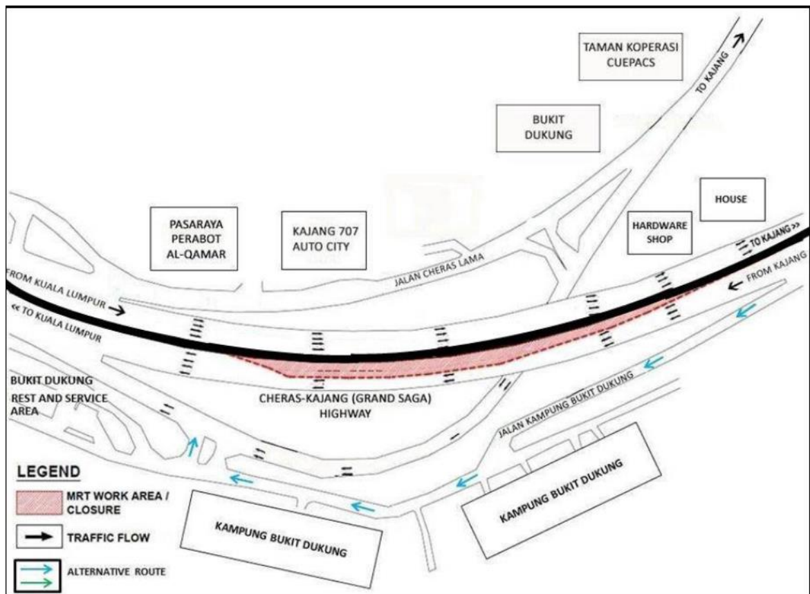
MAP 1: CONTINUATION OF SHORT-TERM LANE CLOSURE AT KM 18.1 CHERAS – KAJANG (GRAND SAGA) HIGHWAY (KL-BOUND)
