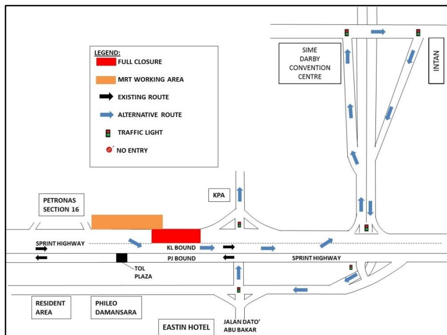
MAP 3: FULL LANE CLOSURE AT KGPA SLIP ROAD AFTER PETRONAS PETROL STATION, SECTION 16, SPRINT HIGHWAY (KL-BOUND)
