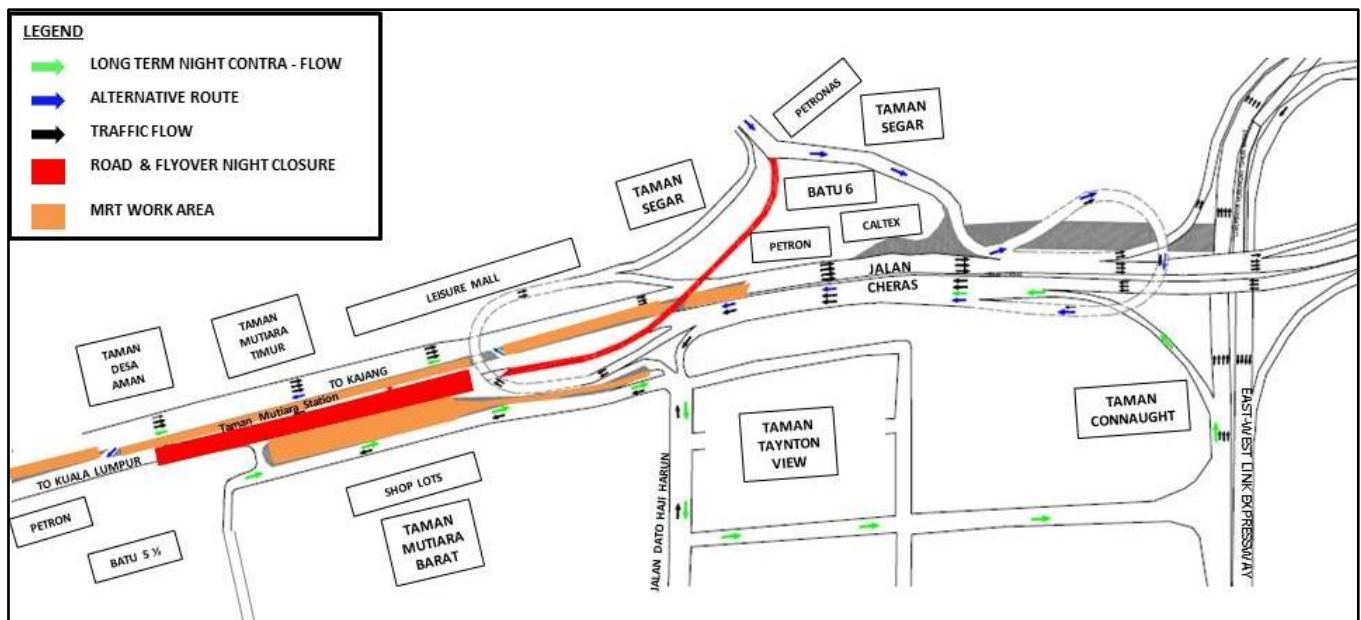
MAP 2: LONG TERM INTERMITTENT NIGHT CONTRA-FLOW AND FLYOVER CLOSURE OPPOSITE LEISURE MALL AT JALAN CHERAS (KL-BOUND)
