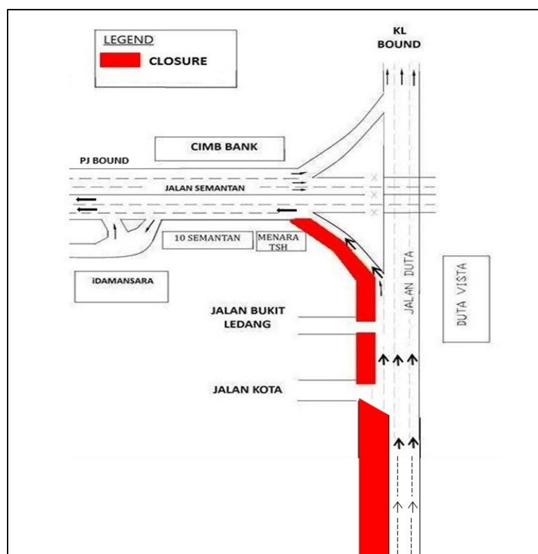
MAP 1: UPDATES ON TRAFFIC MANAGEMENT PLAN FOR MRT CONSTRUCTION WORKS ALONG JALAN DUTA TOWARDS JALAN SEMANTAN (PJ-BOUND)
