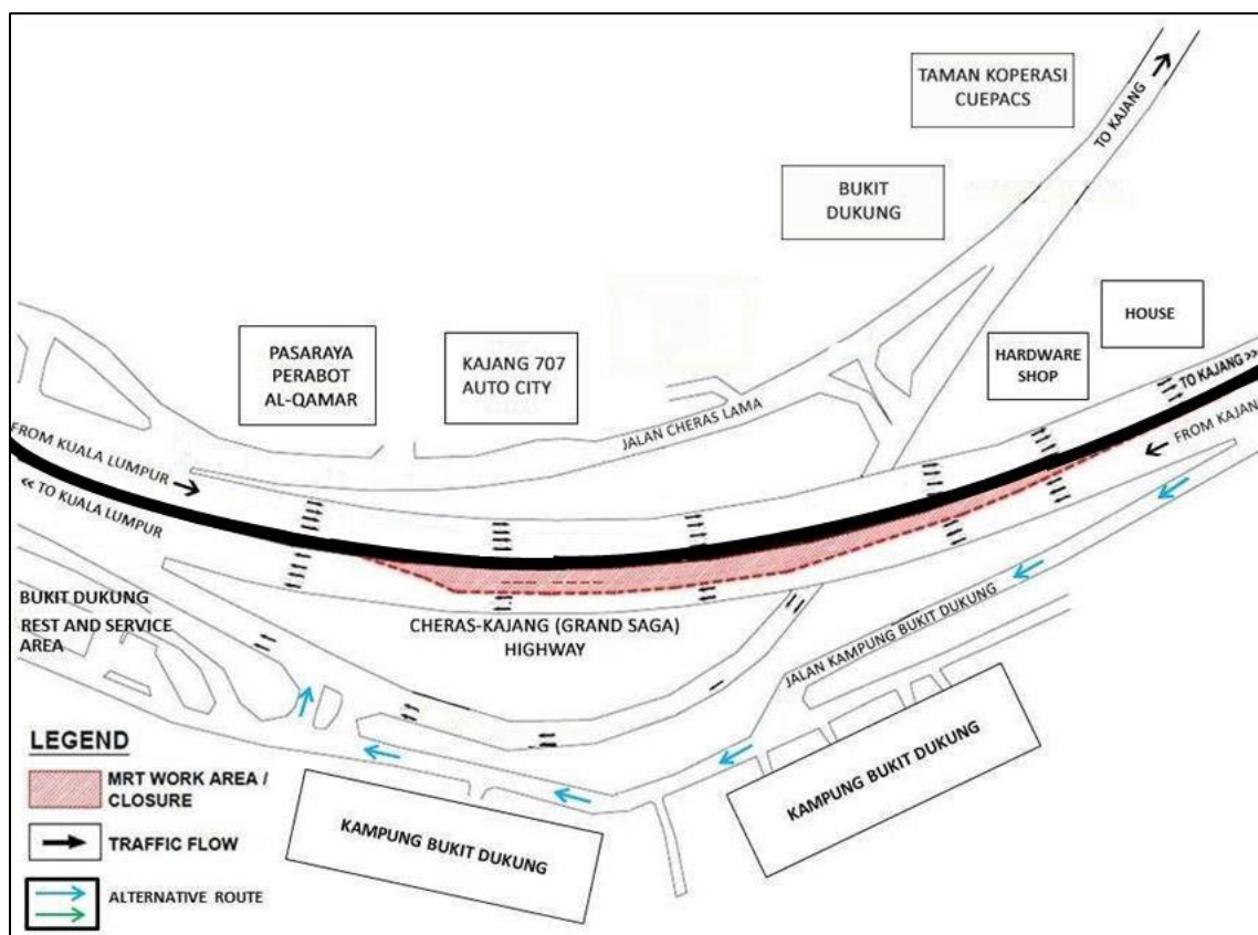
MAP 1: SHORT-TERM LANE CLOSURE AT KM 18.1 CHERAS – KAJANG (GRAND SAGA) HIGHWAY
