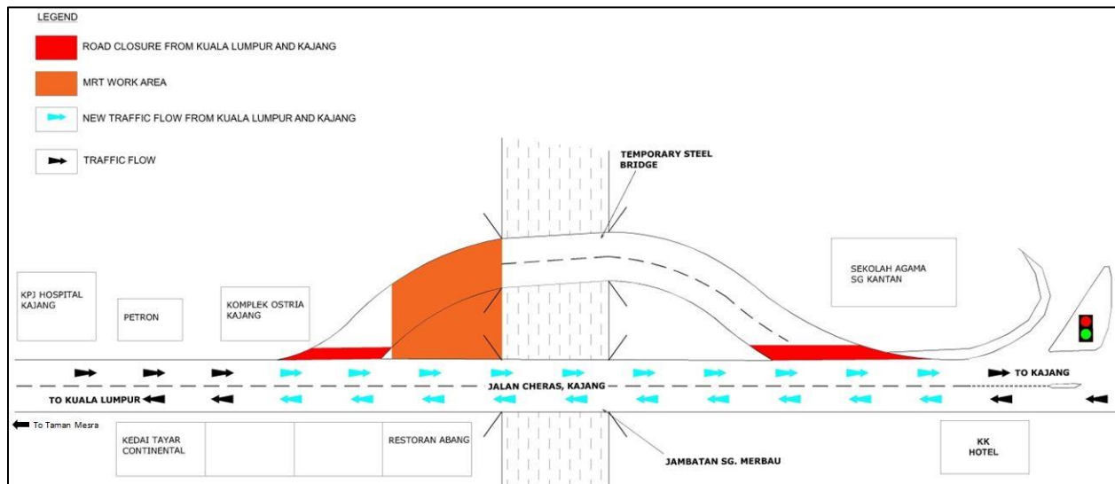
MAP 2: SHORT TERM ROAD CLOSURE AT THE TEMPORARY STEEL BRIDGE AT JALAN CHERAS, KAJANG
