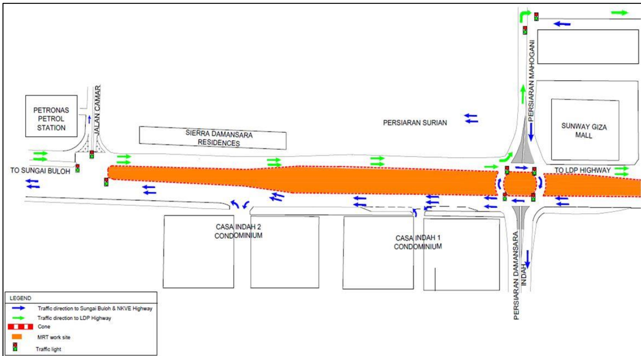
MAP 2: PERMANENT LANE REALIGNMENT AT PERSIARAN SURIAN (SUNGAI BULOH-BOUND)
