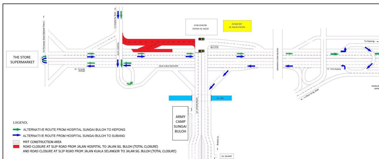
MAP 1A: LONG-TERM ROAD CLOSURE AT SLIP ROAD FROM JALAN HOSPITAL UNTIL THE TRAFFIC LIGHT TO JALAN SUNGAI BULOH (SUBANG-BOUND)/JALAN KUALA SELANGOR (KEPONG-BOUND)
