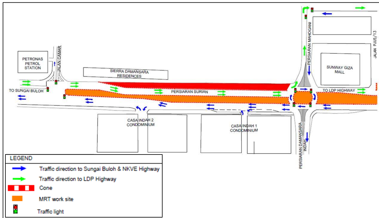
MAP 3: TEMPORARY LANE REALIGNMENT AT PERSIARAN SURIAN (LDP-BOUND)
