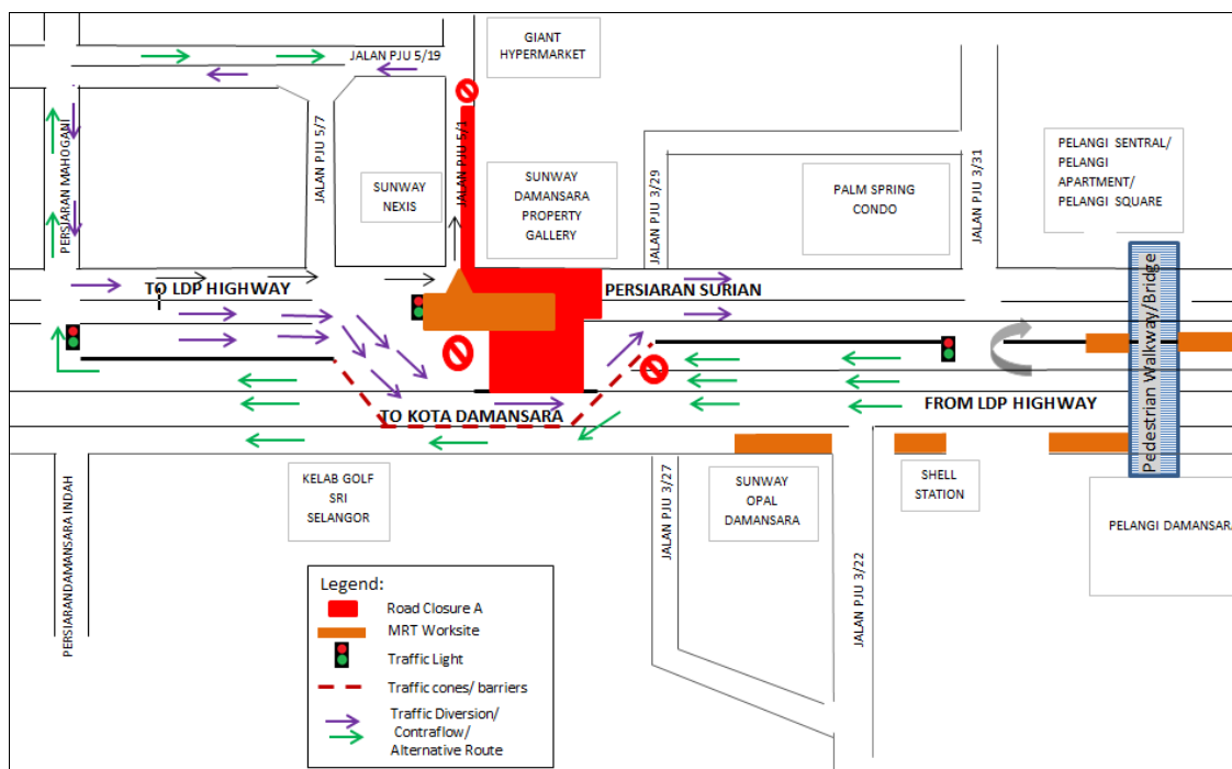
MAP 1, CLOSURE A: LONG-TERM NIGHT TRAFFIC MANAGEMENT PLAN AT PJU 5/1 ALONG PERSIARAN SURIAN (KOTA DAMANSARA-BOUND & LDP HIGHWAY-BOUND)
