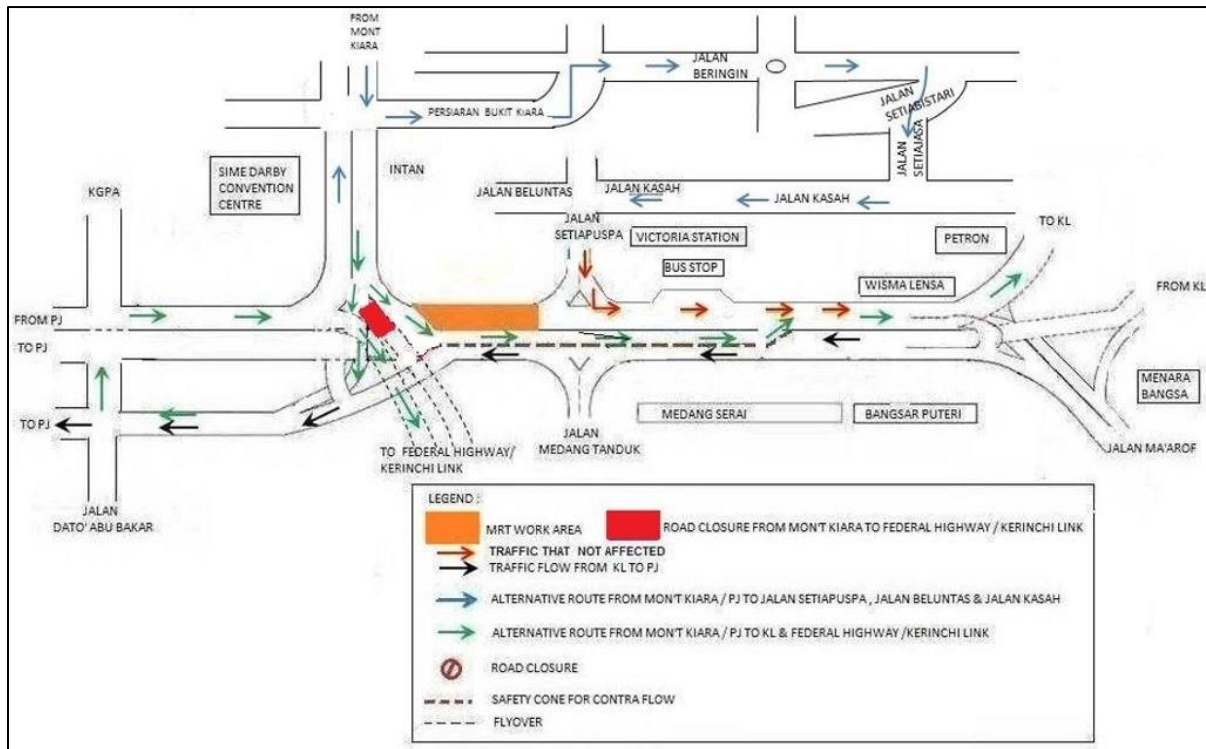
MAP 2: CONTINUATION OF NIGHT TRAFFIC MANAGEMENT PLAN AT SPRINT HIGHWAY FROM KIARA INTERCHANGE TO VICTORIA STATION RESTAURANT (KL-BOUND)
