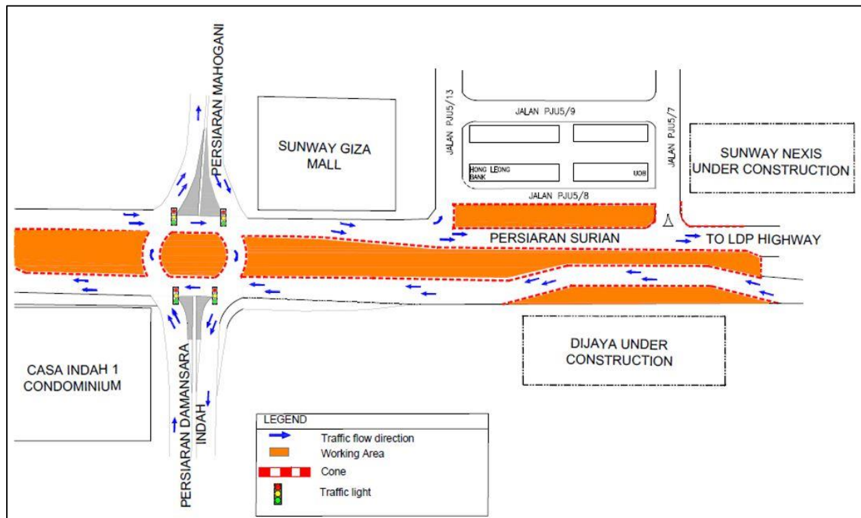
MAP 1: LONG-TERM TEMPORARY LANE REALIGNMENT AT PERSIARAN SURIAN
