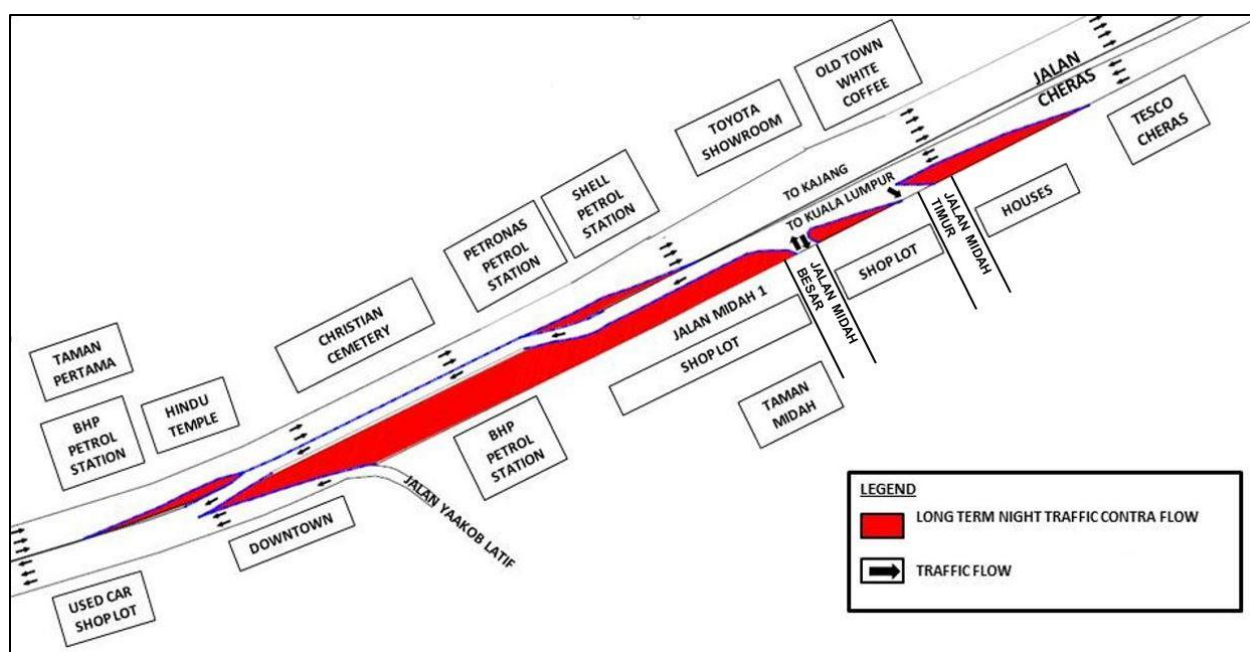
MAP 3: CONTINUATION OF LONG-TERM NIGHT CONTRA-FLOW FROM TAMAN MIDAH TO TAMAN PERTAMA (KL & KAJANG-BOUND)
