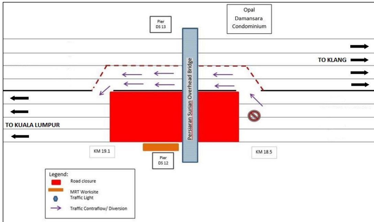
MAP 2, STAGE 2: CONTINUATION OF TRAFFIC DIVERSION AT KM18 NKVE FOR LAUNCHING OF SEGMENTAL BOX GIRDERS (SBGs) FOR THE MRT ELEVATED GUIDEWAY PIERS ON PERSIARAN SURIAN
