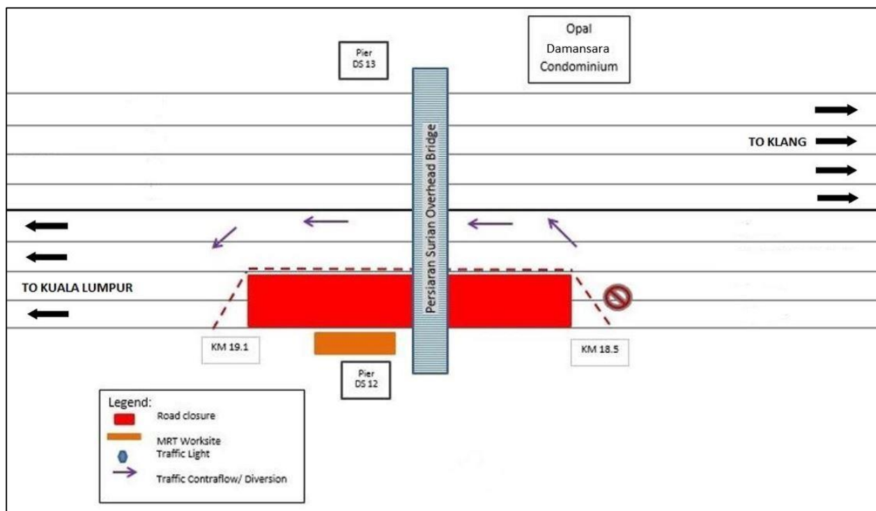
MAP 2, STAGE 1: CONTINUATION OF TRAFFIC DIVERSION AT KM18 NKVE FOR LAUNCHING OF SEGMENTAL BOX GIRDERS (SBGs) FOR THE MRT ELEVATED GUIDEWAY PIERS ON PERSIARAN SURIAN
