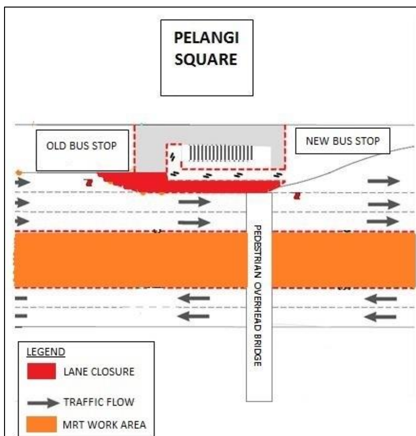
MAP 1: SHORT-TERM CONTINUATION OF SHORT-TERM LANE CLOSURE AT PELANGI SQUARE (LDP HIGHWAY-BOUND)
