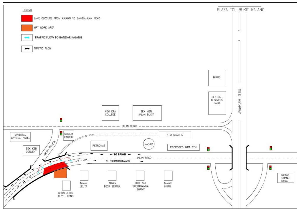
MAP 3: MEDIUM-TERM NIGHT CONTRA-FLOW TRAFFIC AT RAMP OF JALAN REKO, KAJANG
