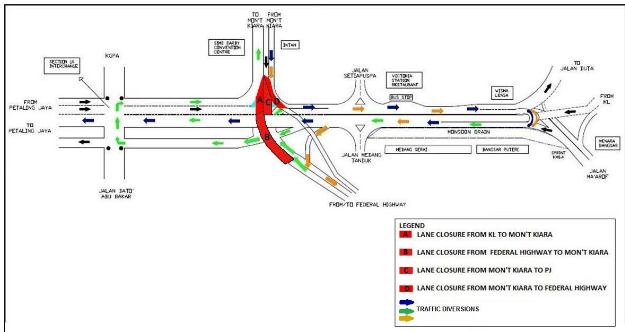
MAP 2: CONTINUATION OF NIGHT CLOSURE AT KIARA INTERCHANGE
