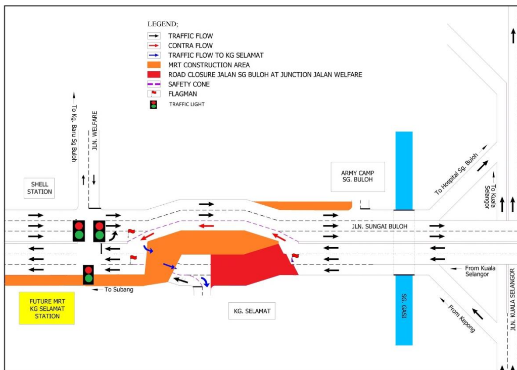
MAP 1: SHORT-TERM NIGHT CONTRA-FLOW TRAFFIC ALONG JALAN SUNGAI BULOH (SUBANG-BOUND)
