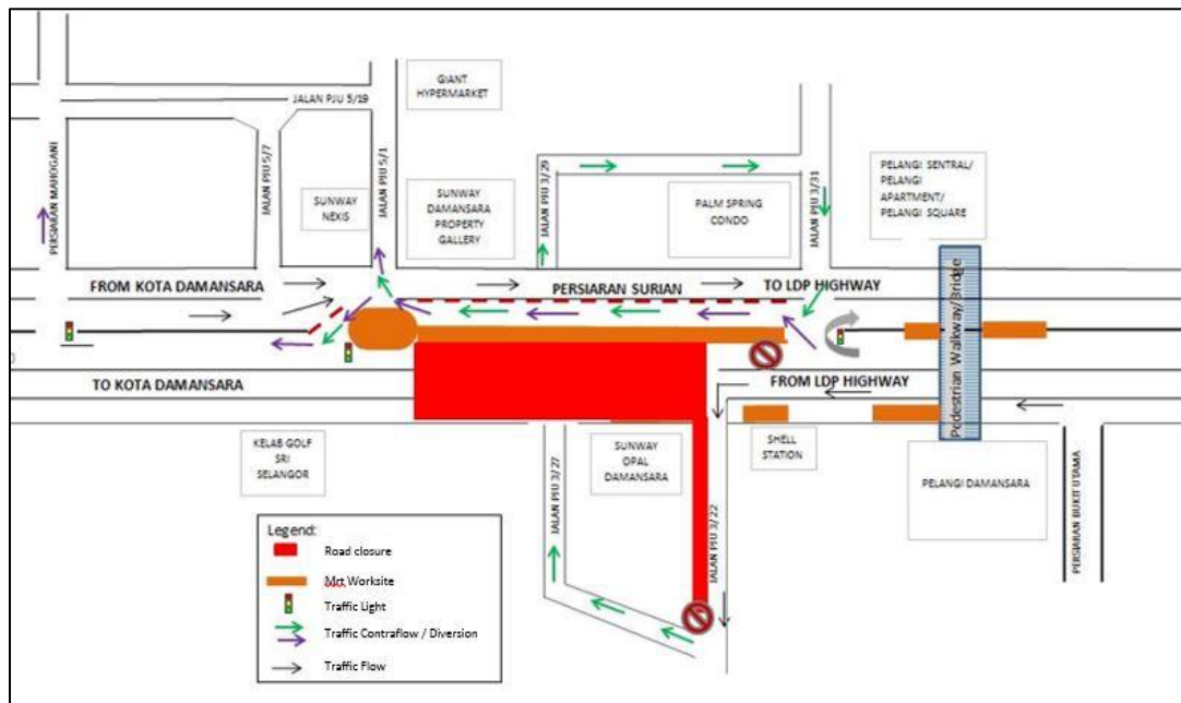
MAP 3: CONTINUATION OF MEDIUM TERM NIGHT CONTRA-FLOW FROM PJU 3/31 TO PJU 5/1 (KOTA DAMANSARA-BOUND) AND LANE CLOSURE AT JALAN PJU 3/22 (PERSIARAN SURIAN-BOUND)
