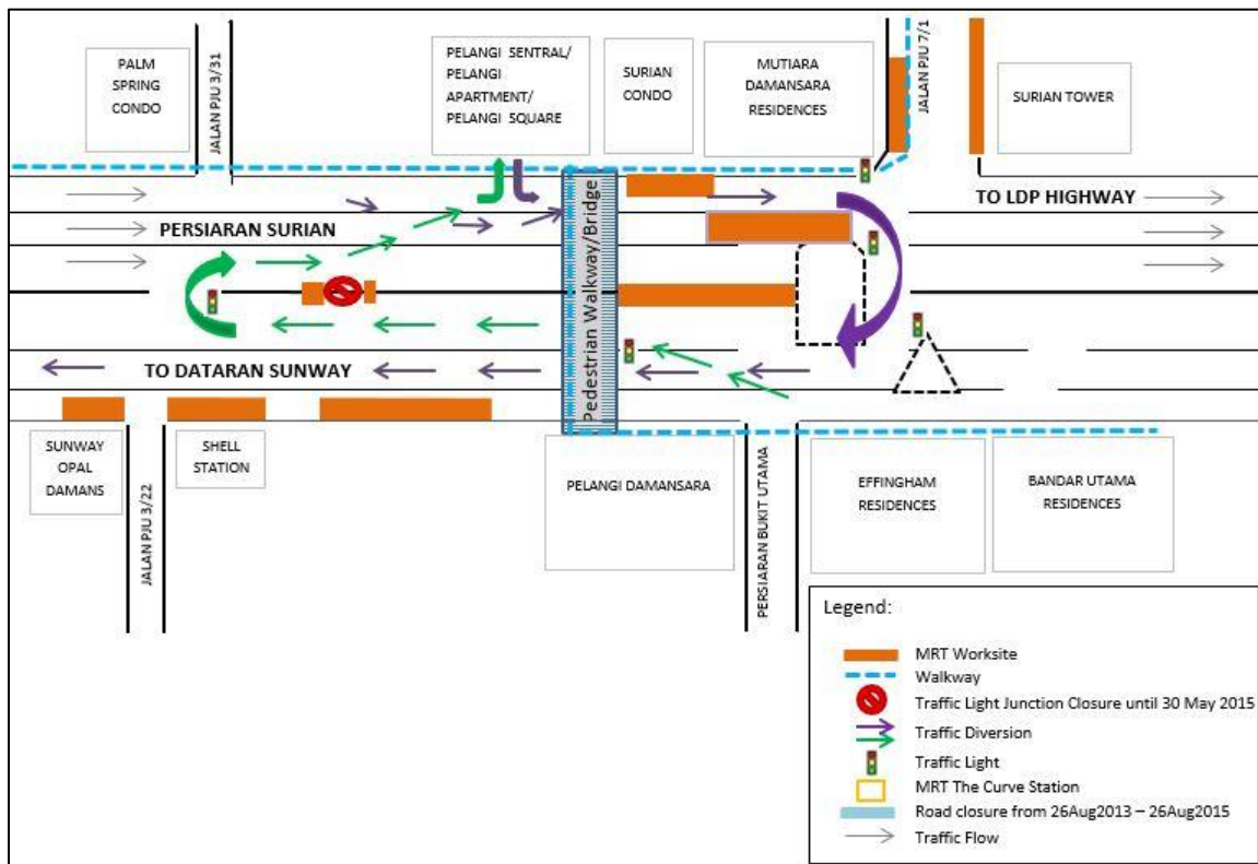
MAP 2: CONTINUATION OF TRAFFIC LIGHT JUNCTION CLOSURE AT THE INTERSECTION OF PERSIARAN SURIAN AND PELANGI SENTRAL
