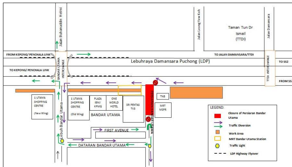
MAP 1: SHORT TERM ROAD CLOSURE OF PERSIARAN BANDAR UTAMA (ALONG LDP HIGHWAY)
