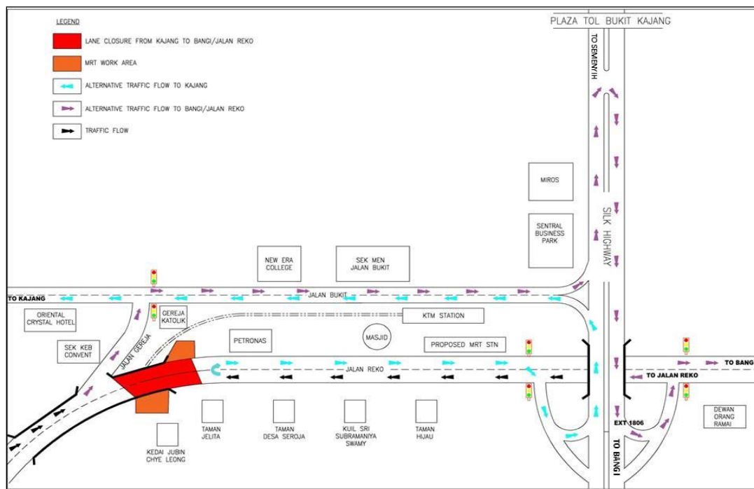
MAP 3: NIGHT ROAD CLOSURE AT JALAN REKO, KAJANG (BANGI-BOUND & BANDAR KAJANG-BOUND)
