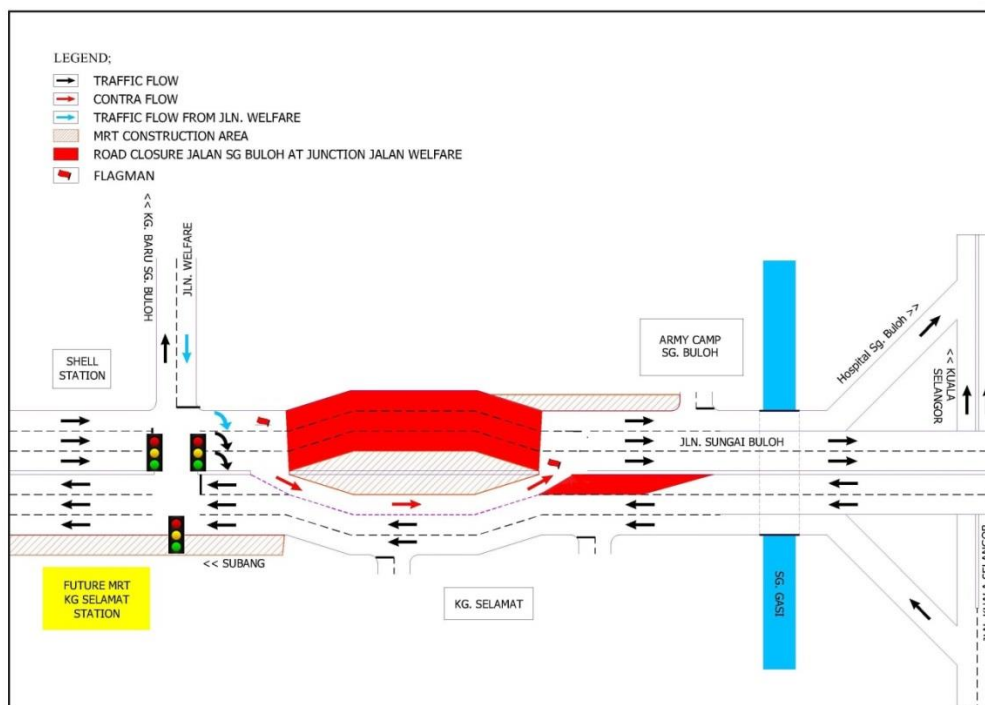
MAP 2: MEDIUM TERM NIGHT CONTRA-FLOW TRAFFIC ALONG JALAN SUNGAI BULOH (KUALA SELANGOR-BOUND)
