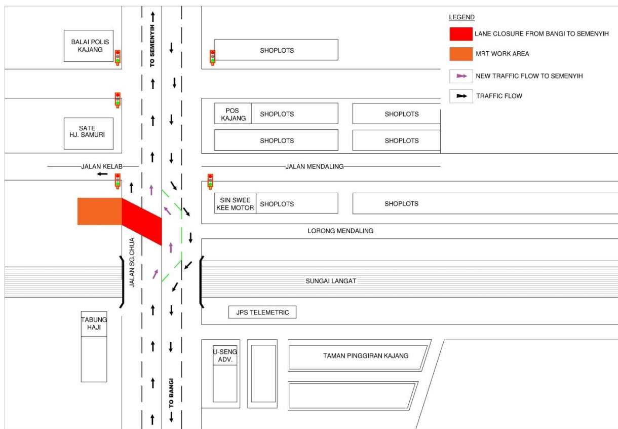
MAP 4; STAGE 1: SHORT TERM NIGHT CONTRA-FLOW AT JALAN SUNGAI CHUA, KAJANG (BANGI-BOUND & SEMENYIH-BOUND)
