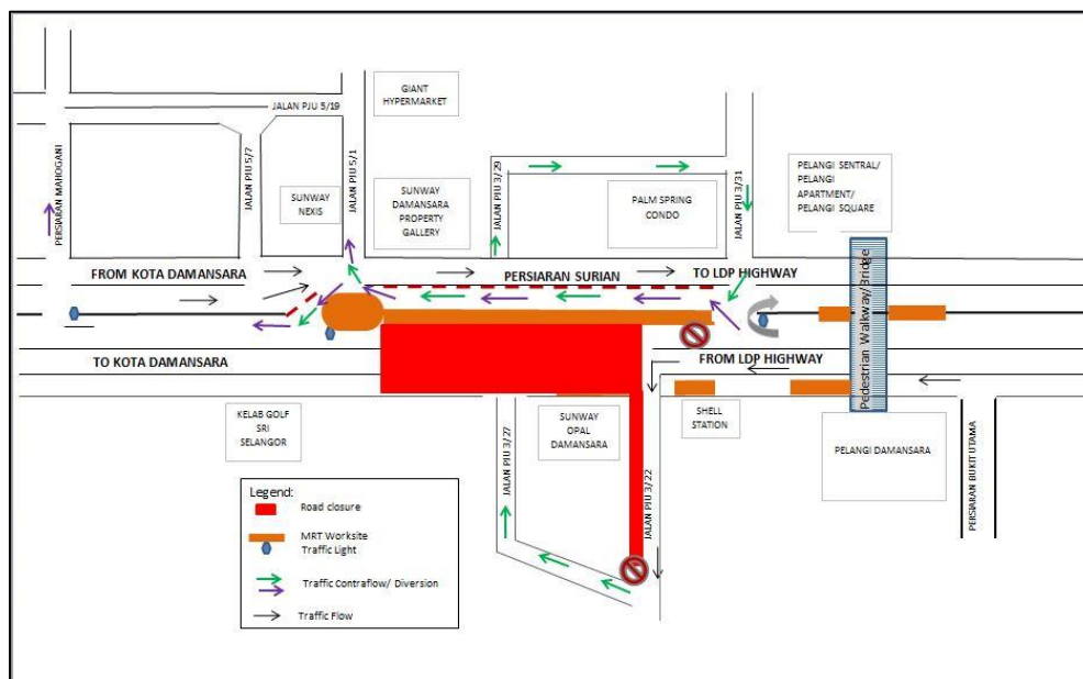
MAP 1: MEDIUM TERM NIGHT CONTRA-FLOW FROM PJU 3/31 TO PJU 5/1 (KOTA DAMANSARA-BOUND) AND LANE CLOSURE AT JALAN PJU 3/22 (PERSIARAN SURIAN-BOUND)
