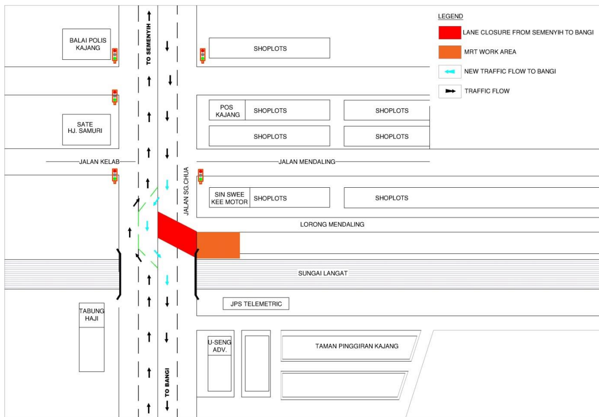
MAP 4; STAGE 2: SHORT TERM NIGHT CONTRA-FLOW AT JALAN SUNGAI CHUA, KAJANG (BANGI-BOUND & SEMENYIH-BOUND)
