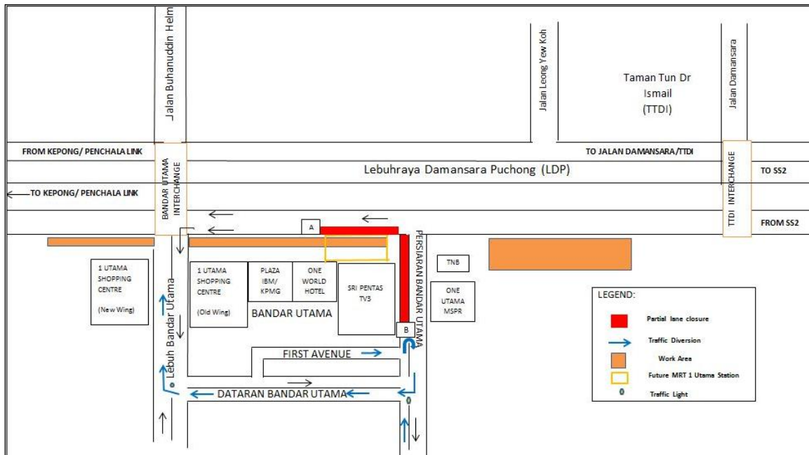
MAP 5: CONTINUATION OF LONG-TERM NIGHT TRAFFIC MANAGEMENT PLAN AT PERSIARAN BANDAR UTAMA (LDP HIGHWAY; KEPONG-BOUND)
