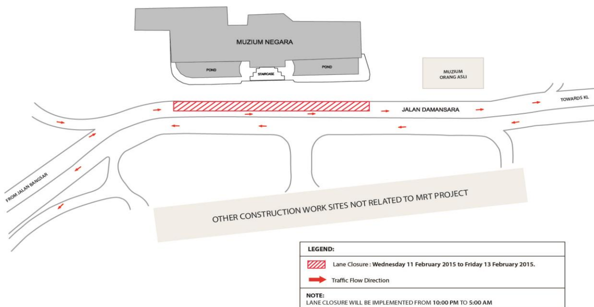
MAP 1: NIGHT LANE CLOSURE ON JALAN DAMANSARA
