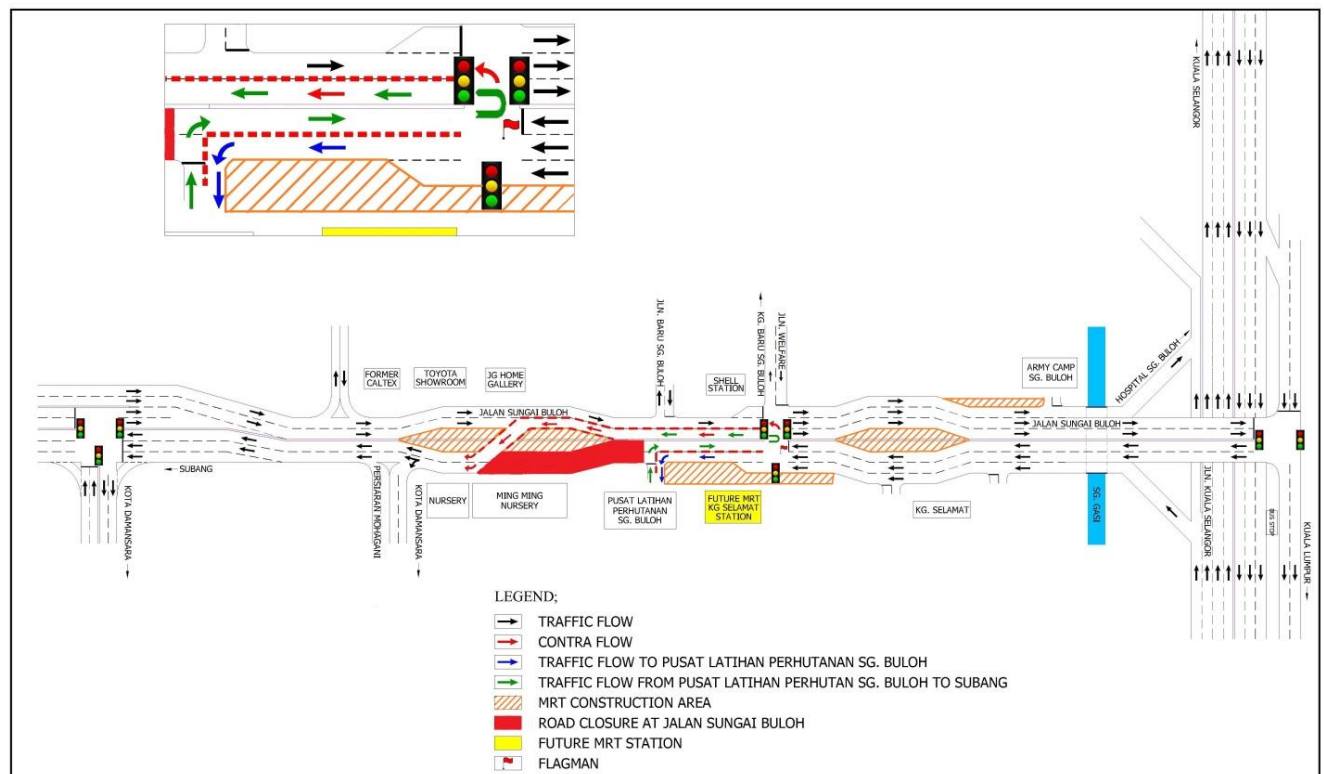
MAP 2: SHORT-TERM NIGHT CONTRA-FLOW TRAFFIC ALONG JALAN SUNGAI BULOH IN FRONT OF MING MING NURSERY (SUBANG-BOUND)
