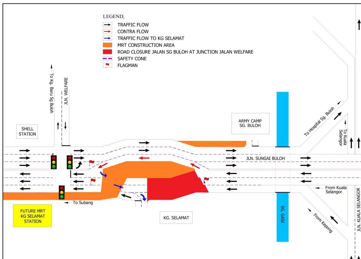
MAP 1: SHORT-TERM NIGHT CONTRA-FLOW TRAFFIC ALONG JALAN SUNGAI BULOH IN FRONT OF KAMPUNG SELAMAT (SUBANG-BOUND)
