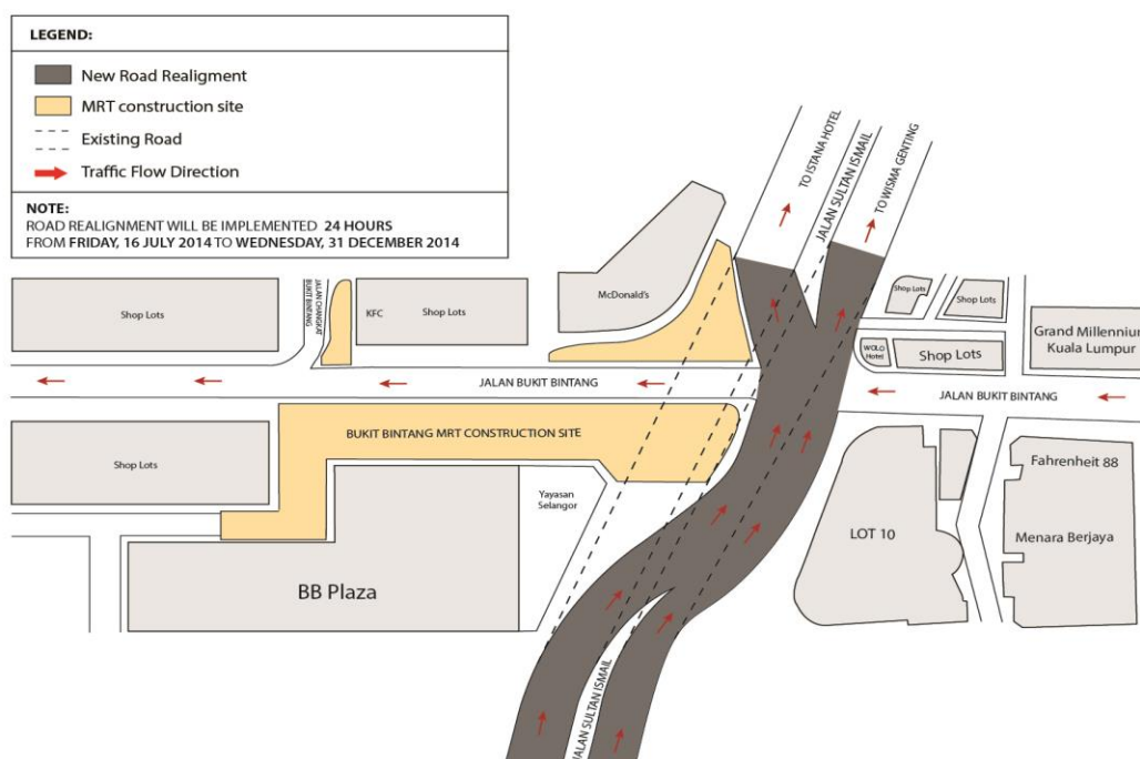
LONG-TERM ROAD REALIGNMENT AT JALAN BUKIT BINTANG & JALAN SULTAN ISMAIL INTERSECTION
