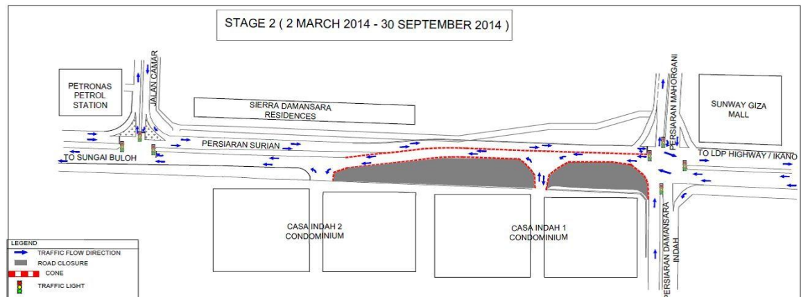
MAP 2: TEMPORARY TRAFFIC DIVERSION AT PERSIARAN SURIAN
