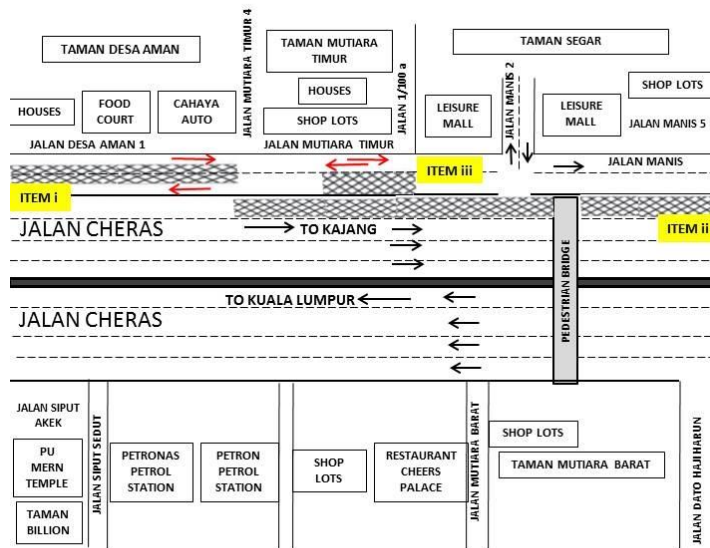
TEMPORARY LANE CLOSURE/ MRT WORK AREA (From 17 June 2013 to 7 October 2013)
